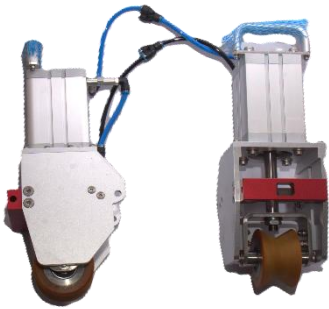
U000-0001 Pneumatic lift-off device Suitable for all devices in the U series enables the device to be lifted to pass over obstacles CTN: 90249000 Country of origin: Germany
