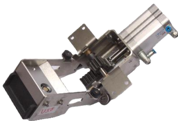
U000-0003 Pneumatic sensor opener Suitable for U58 enables the lower sensor to be opened to pass over obstacles CTN: 90249000 Country of origin: Germany
