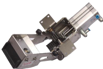
U000-0004 Pneumatic sensor opener Suitable for U83 enables the lower sensor to be opened to pass over obstacles CTN: 90249000 Country of origin: Germany
